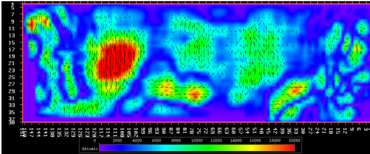
Figure 4. Map of seismic anisotropy in the Upper Coal indicated in Figure 3. Hot colors indicate higher levels of seismic anisotropy. The lines on the image indicate the orientation of the anisotropy. North is to the top of the figure.
