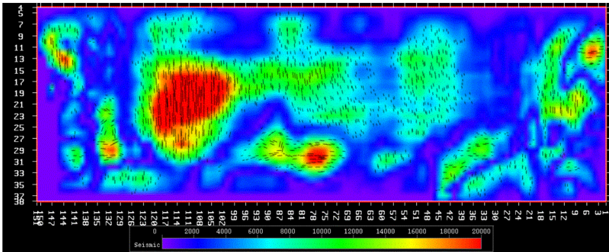
Figure 5. Map of seismic anisotropy in the Middle Coal indicated in Figure 3. Hot colors indicate higher levels of seismic anisotropy. The lines on the image indicate the orientation of the anisotropy. North is to the top of the figure.
