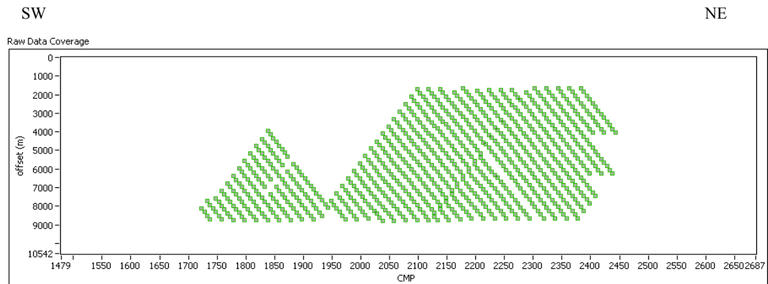
Figure 4 Common midpoint (CMP) versus offset plot. The Earth's impulse response has been determined for each point over a lateral range of 15 km and an offset range of 2 km to 9 km. Distance along the profile is related to the CMP number through distance = (CMP/10-101) \times 200 m.
