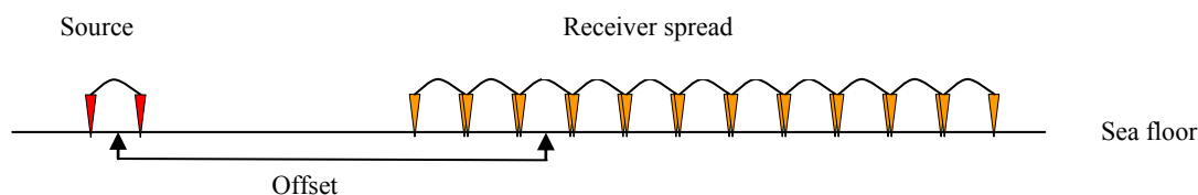
Figure 1 Acquisition geometry for OBC transient EM surveying.
