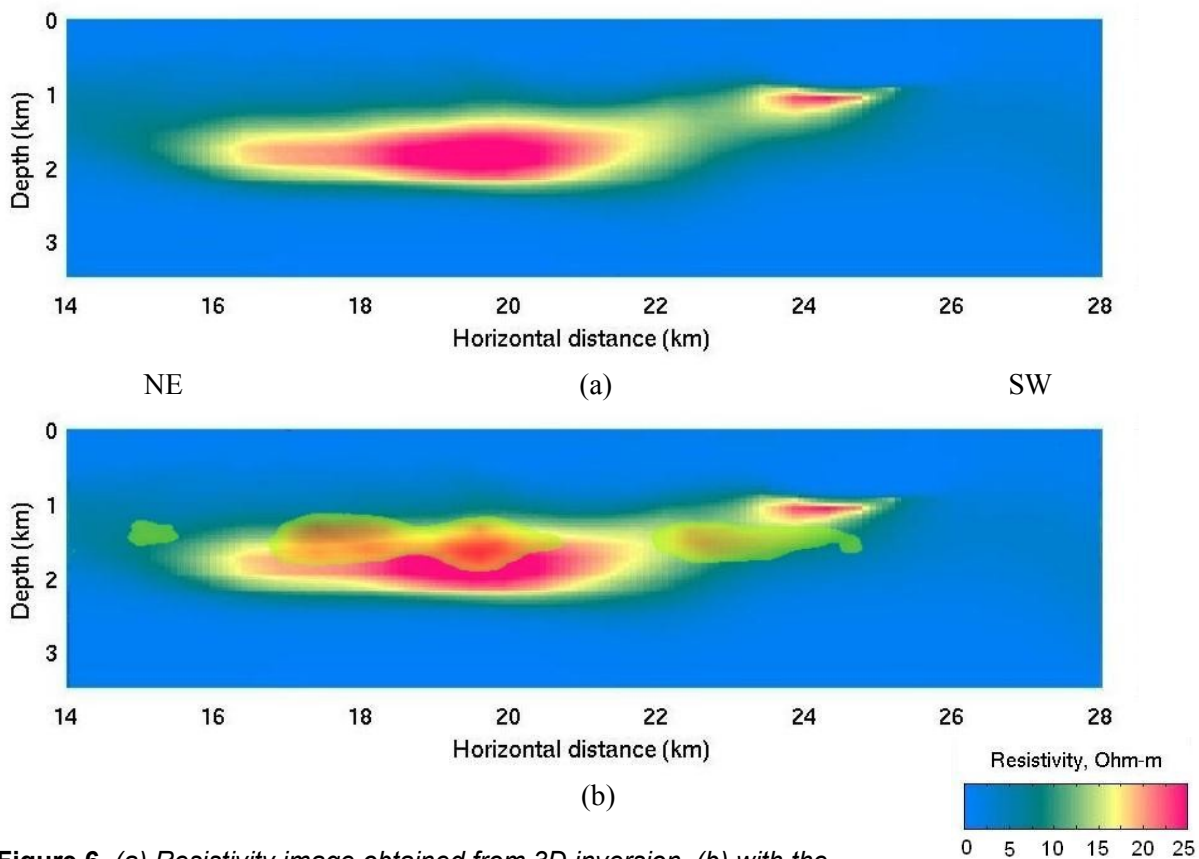
Figure 6 (a) Resistivity image obtained from 3D inversion, (b) with the > 3 \Omega\text{m} features from the collated 1D resistivity image superimposed upon it.
