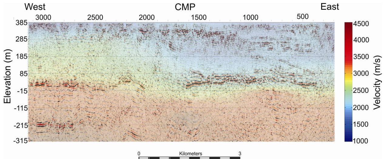
Figure 3: Final Prestack depth migrated seismic overlaid with the travelt ime inversion velocities.
