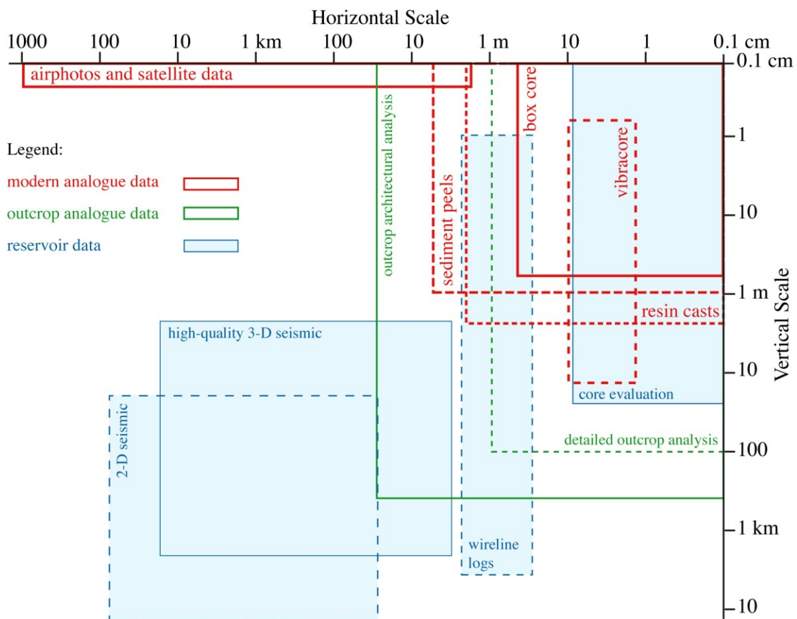
Figure 1 – A schematic representation of the horizontal and vertical scales of modern, outcrop, and subsurface reservoir datasets. Modern datasets provide high-resolution sedimentological, ichnological, and morphological data at a broad range of lateral scales, but tend to be vertically restricted. Outcrop, and more so, subsurface datasets cover a greater vertical range, but are commonly much lower resolution than modern datasets. As well, subsurface and outcrop data provide much lower resolution data in the horizontal plane.
