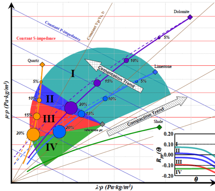
Figure 2: LMR crossplot showing effects of lithology, porosity and fluids. After Hoffe et al (2008).
