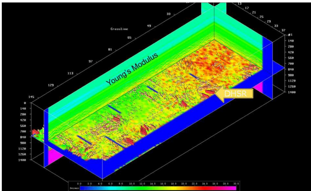
Figure 3: Young's Modulus Cube (Gray, 2010)
