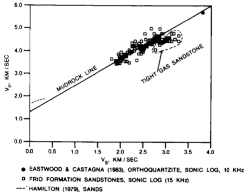
Figure 1: Sonic Log Velocities in Sandstone (Castagna et al, 1985)
