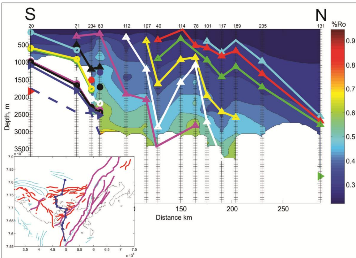
Figure 3: North-south cross-section through Beaufort-Mackenzie Basin (blue line on inset map) showing %Ro trends with respect to various stratigraphic successions (coloured lines on cross-section).
