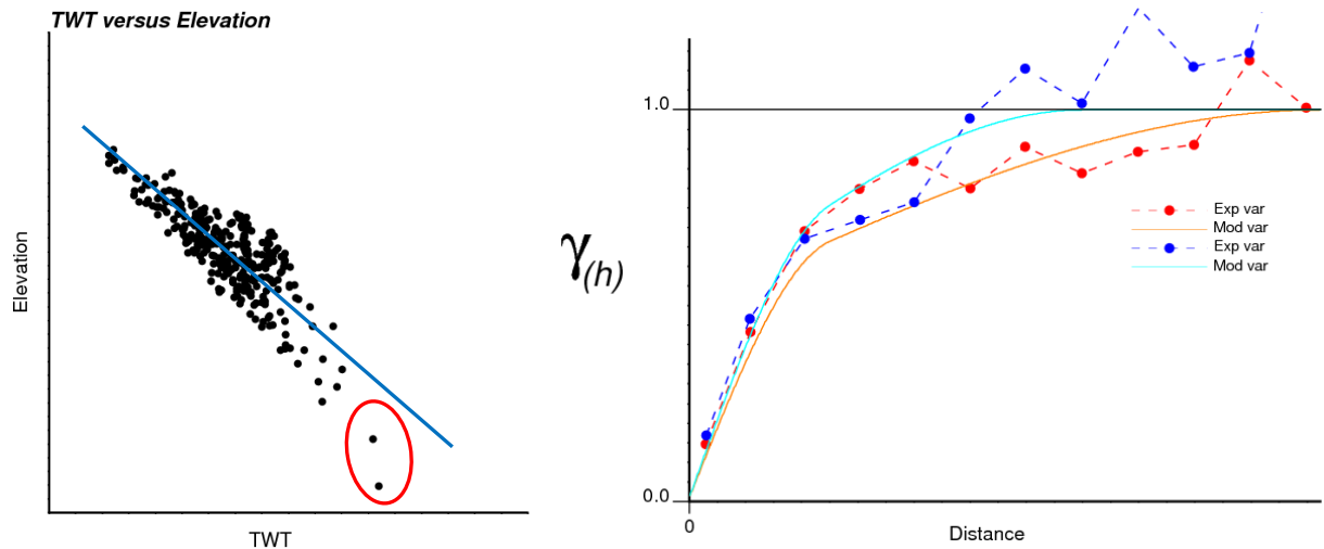
Figure 6: A typical Two-way-time versus well marker elevation showing the linear regression line and the outliers (left), and typical normalized directional experimental and modeled variograms with two nested structures that show anisotropy in the spatial correlation of the residuals.
