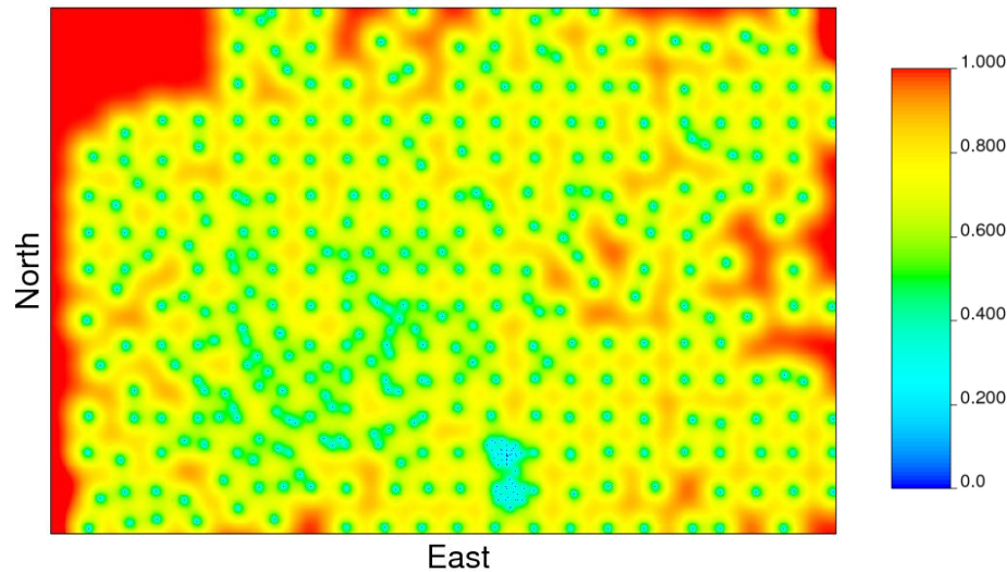
Figure 3: The normalized uncertainty map based on the application of OK with well markers only.
